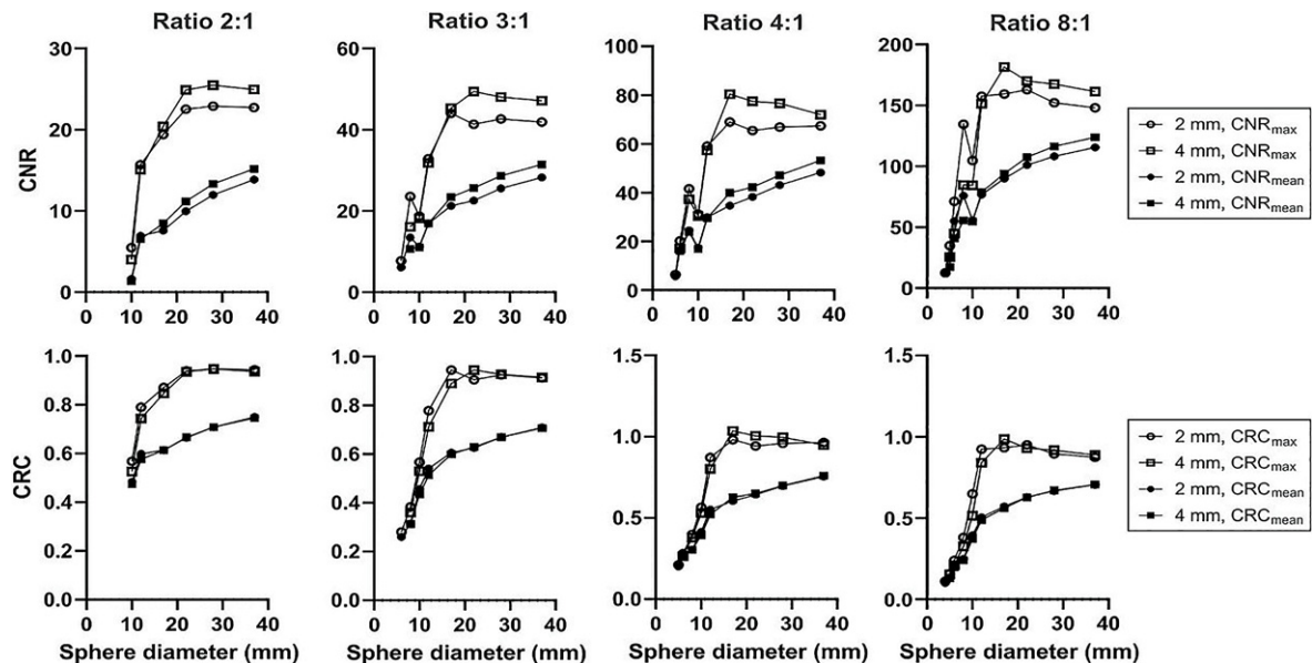
FIGURE 2. Measurements of contrast-to-noise ratio ( CNR_{max/mean} ) (top row) and contrast recovery coefficient ( CRC_{max/mean} ) (bottom row) in all NEMA body and the Micro Hollow-Sphere phantom spheres for all radioactivity concentration ratios with 2 mm and 4 mm in-line pixel size.
